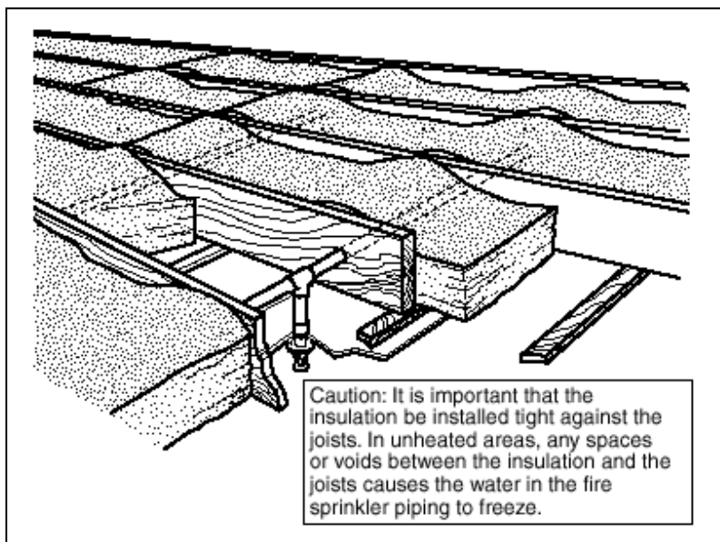
Insulation Recommendation – Arrangement 1
