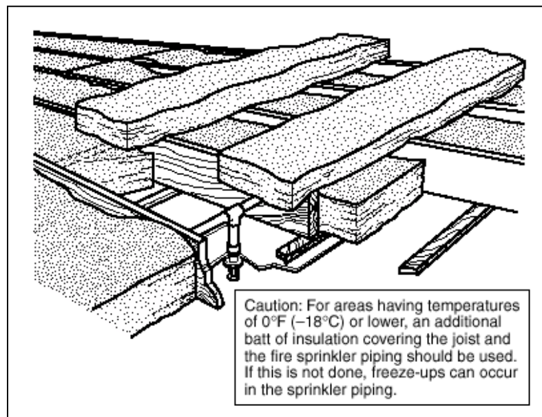
Insulation Recommendation – Arrangement 2
