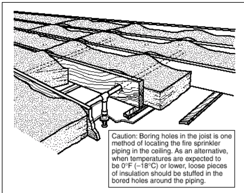
Insulation Recommendation – Arrangement 3
