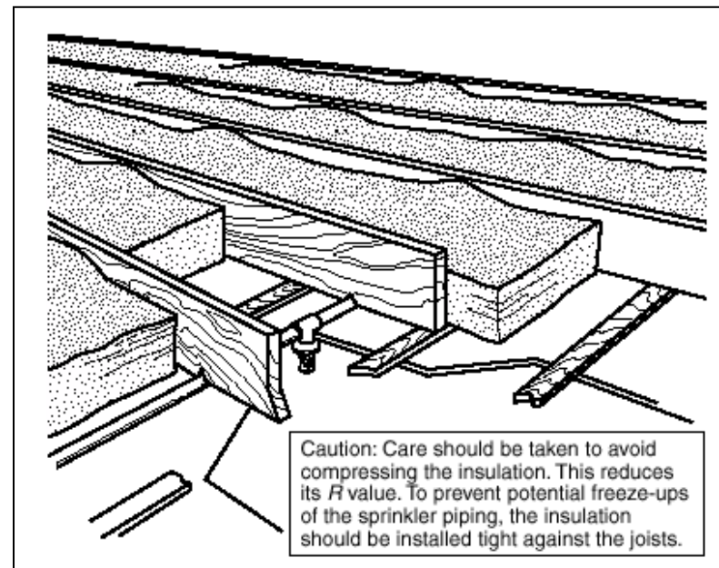
Insulation Recommendation – Arrangement 4
