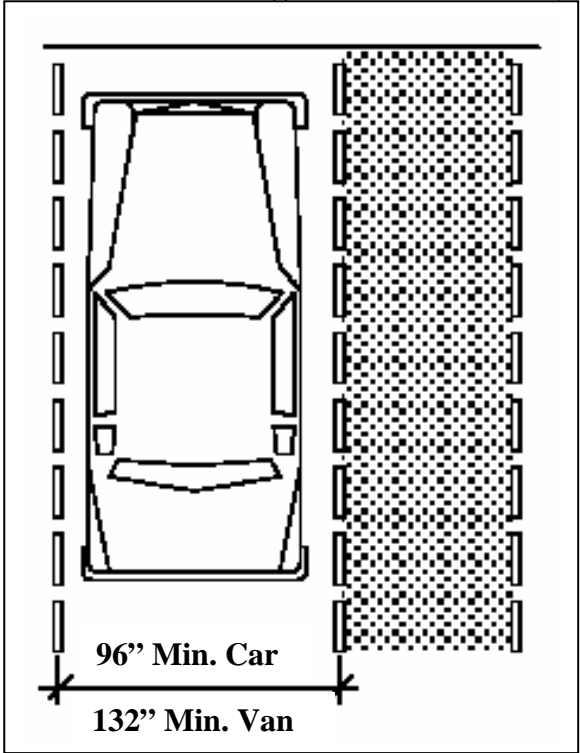
EXAMPLE HANDICAP PARKING SPACE (FOR REFERENCE ONLY)
